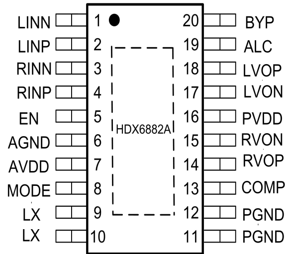
TSSOP20 PACKAGE TOPVIEW
